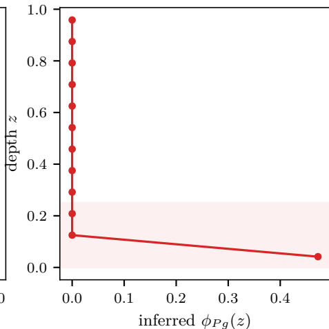
Inverse: 40% detachment \rightarrow Pg at substratum
