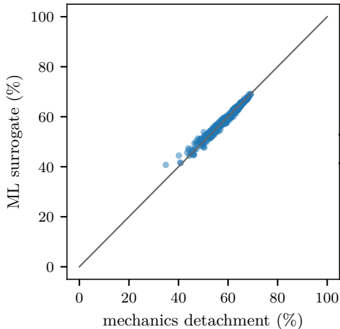
Forward surrogate: R^2 = 0.973
