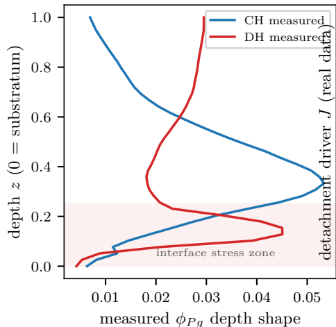
Real FISH depth profiles (endpoint)
