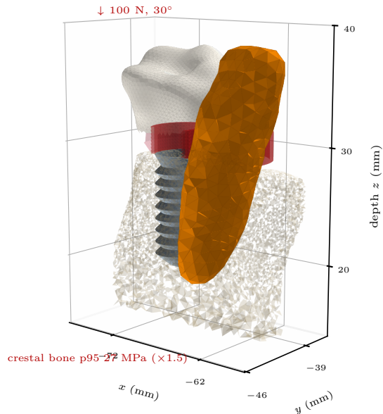
(B) restored: crown + gingiva (load at occlusal table)
