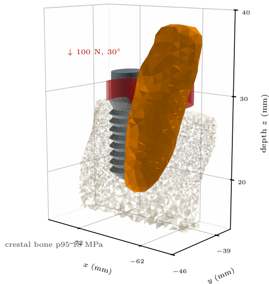
(A) bare screw + abutment (load at platform)
