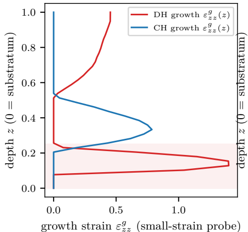
CLSM growth eigenstrain (endpoint)
