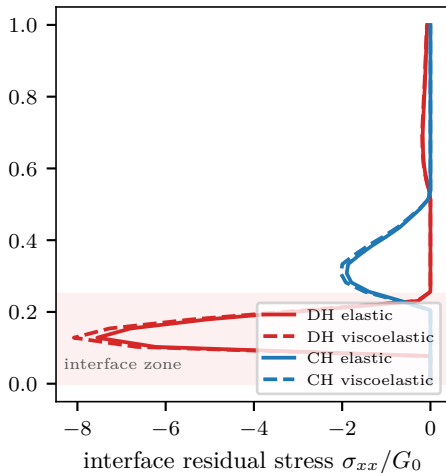
Volumetric-dominated: VE relaxation does not relieve it ( De \approx 5 \times 10^{-4} , g_\infty = 0.05 , K/G \approx 10 )
