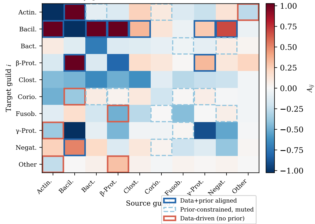
(A) Mean A_{ij} (gLV \alpha=0.25 , 10-fold LOO)
