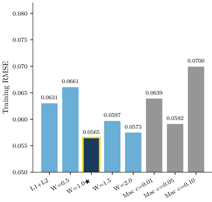
(A) Training RMSE
