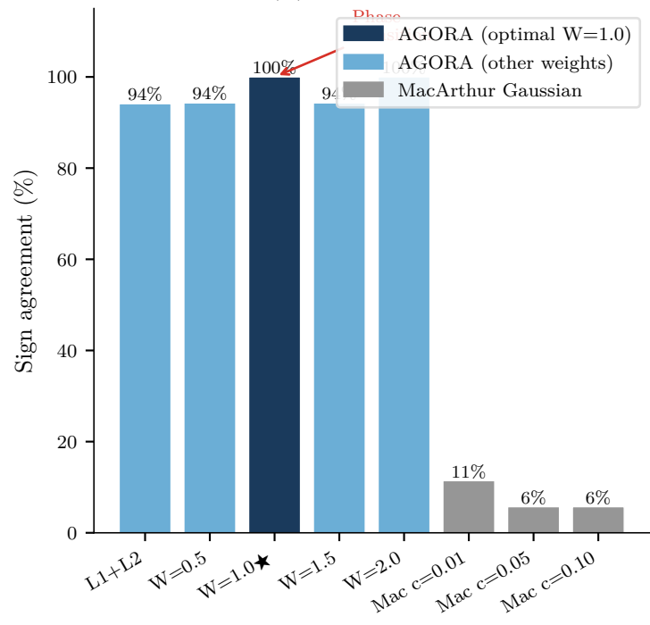
(C) Sign agreement
