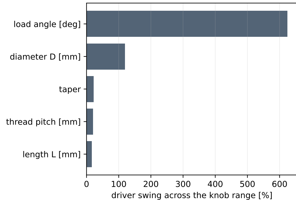
(C) which knob moves the driver most
