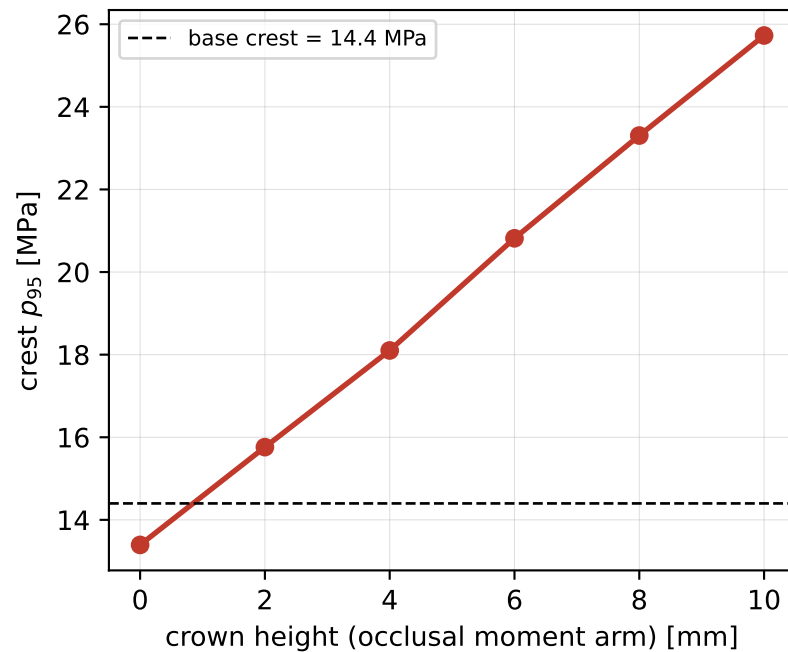
(B) moment arm raises the driver
