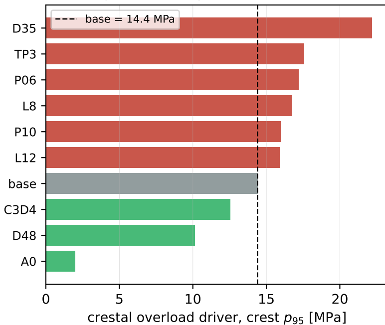
(A) designs ranked by overload driver
