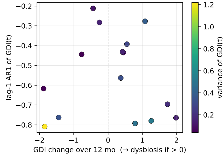
(C) data: AR1 vs trajectory Spearman \rho = -0.07 , p = 0.80 ( n = 15 )
