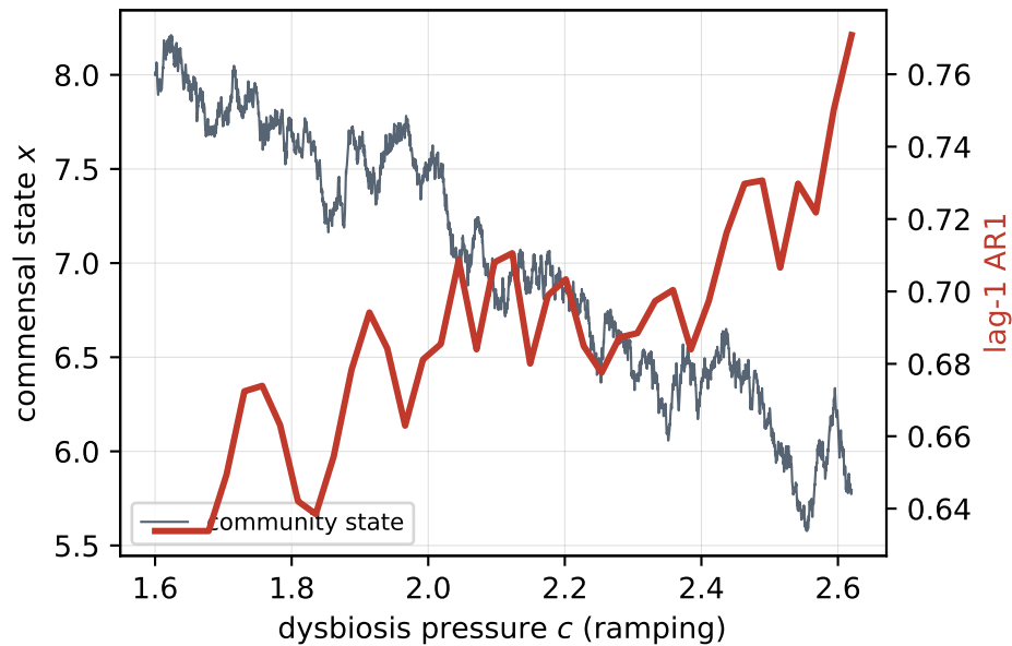
(A) model: state declines, AR1 rises
