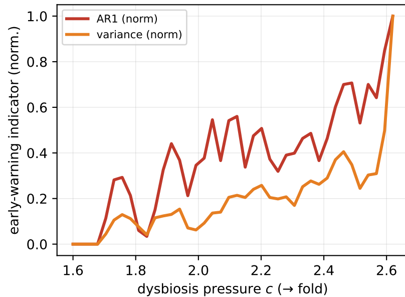
(B) CSD: AR1 & variance rise before the tip
