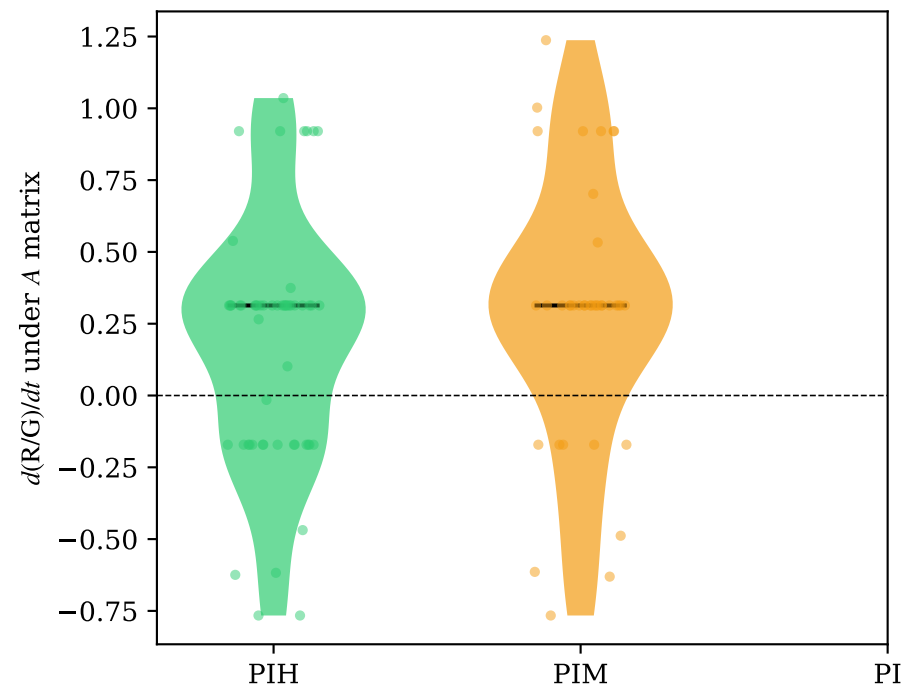
(A) A-matrix velocity R/G rate \rho=0.16 p=0.130
