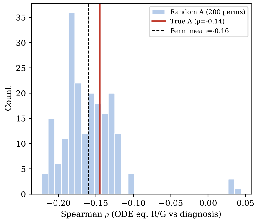
(B) A matrix permutation test p=0.325 (true A vs random)
