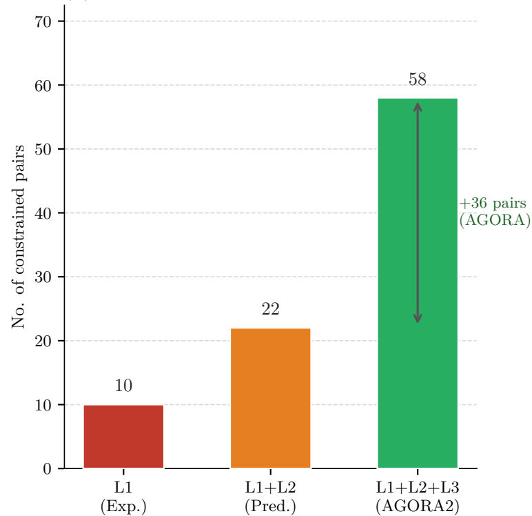
(B) Constrained pairs by prior layer
