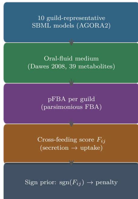
(A) AGORA2 FBA pipeline
