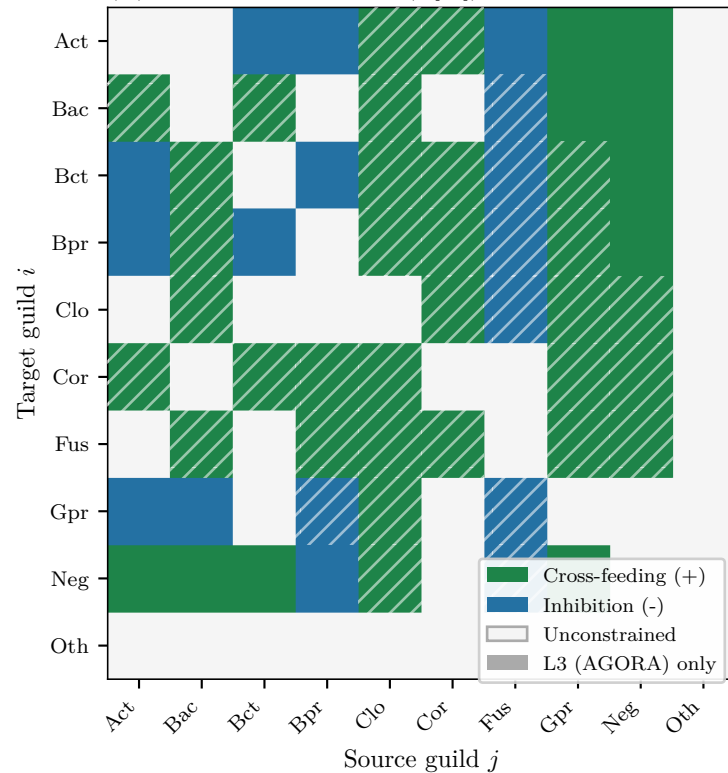
(C) Sign prior matrix \text{sgn}(F[i,j])
