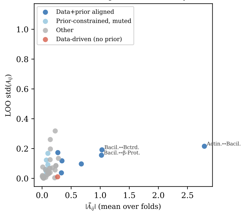
(B) Interaction strength vs LOO variability
