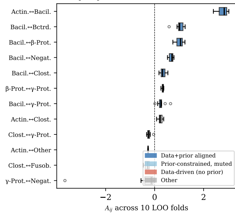
(C) Top 12 pairs: fold-to-fold distribution
