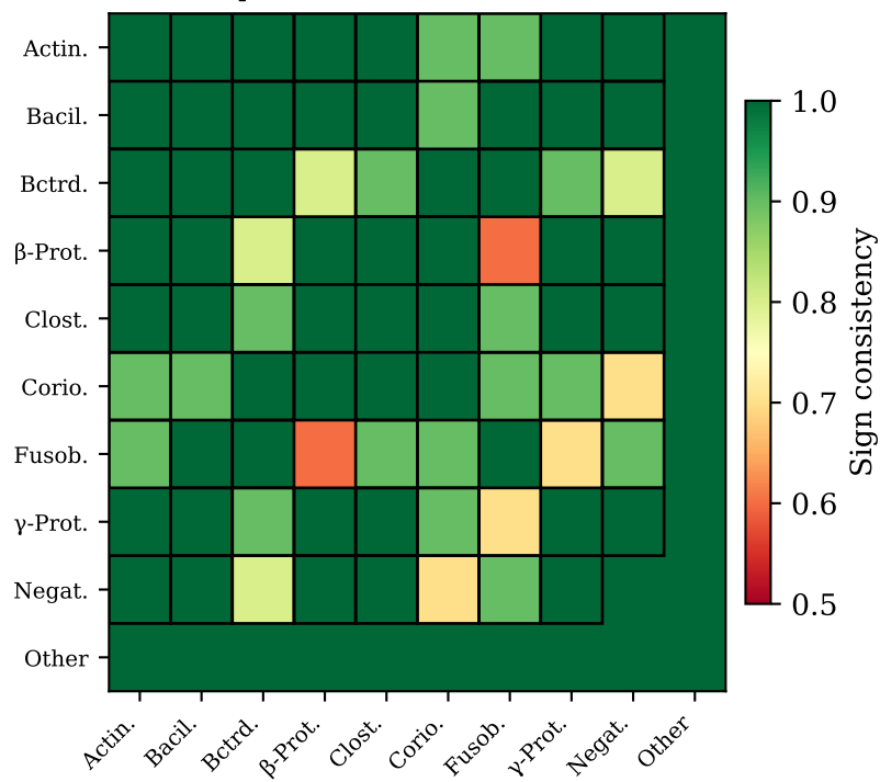
(A) LOO sign consistency (boxed = prior constrained)
