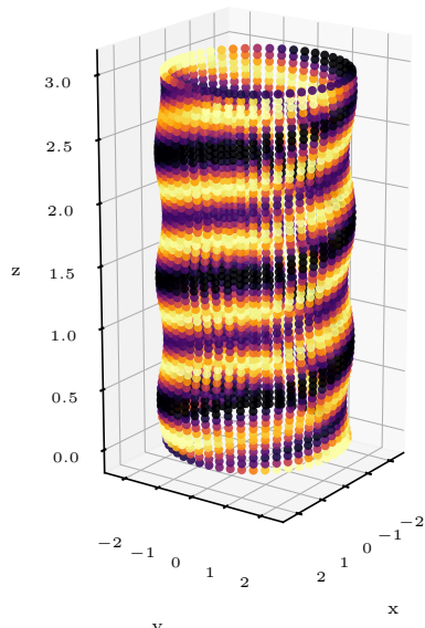
(A) Helical screw interface \sigma_{vM}
