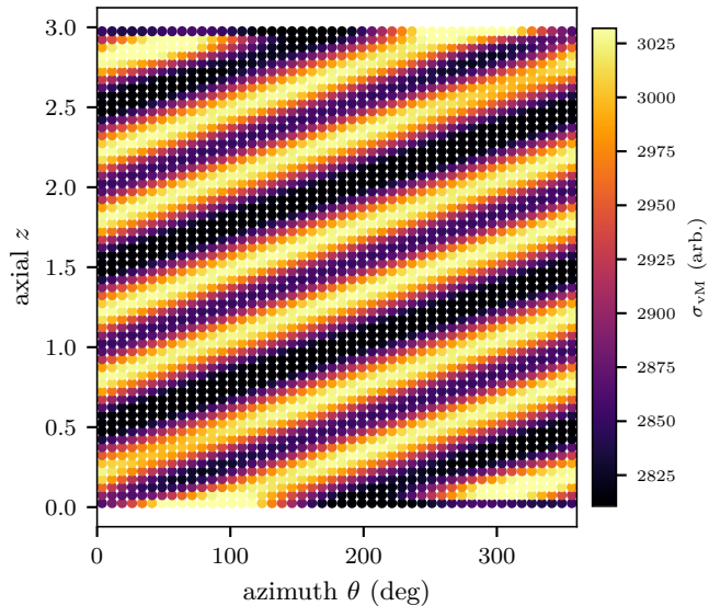
(B) Unrolled interface (helical bands)
