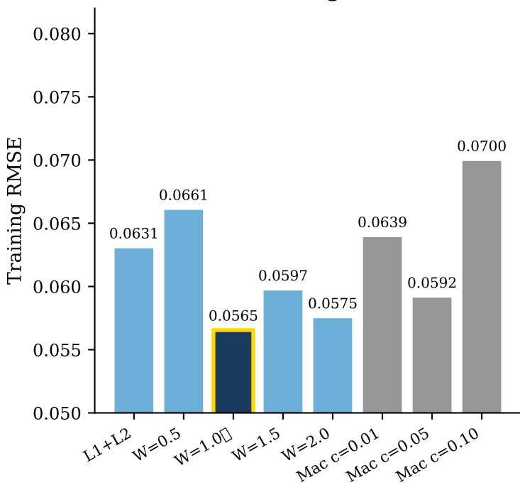
(A) Training RMSE
