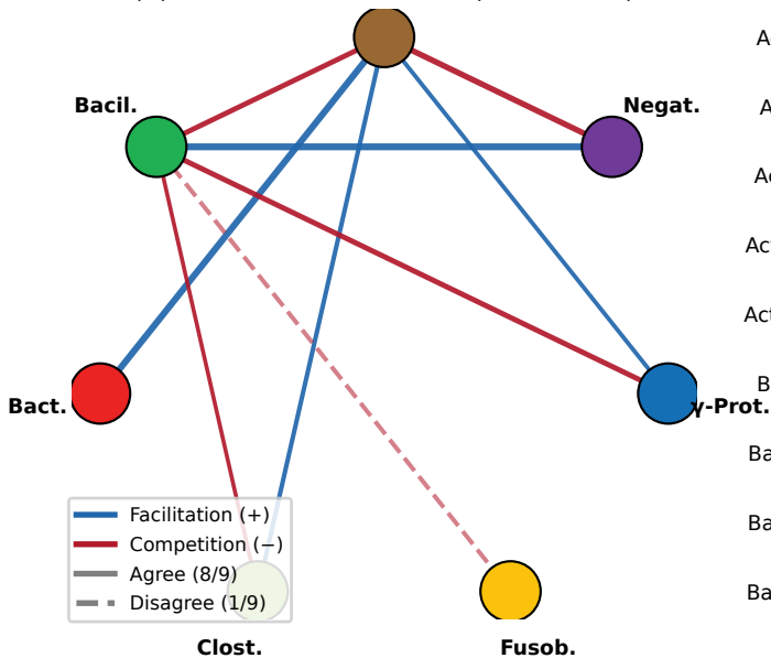
(A) Cross-cohort backbone (theta = 0.1)
