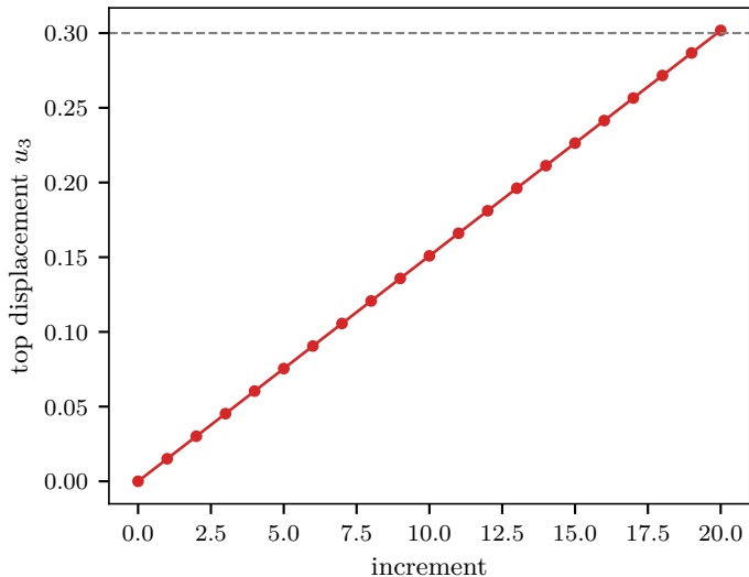
Finite-strain free-swelling: u_3 \rightarrow \lambda_z - 1 (Abaqus)
