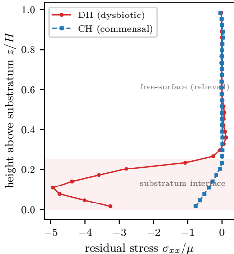
Substratum-interface residual stress: DH \gg CH (peak 6.4\times , mean 10\times )
