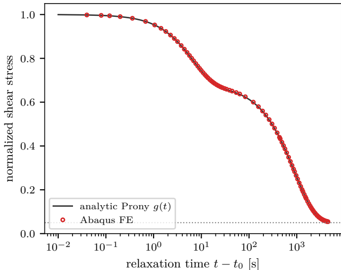
Biofilm stress relaxation (Burgers \rightarrow Prony, RMS 9\times 10^{-4} )
