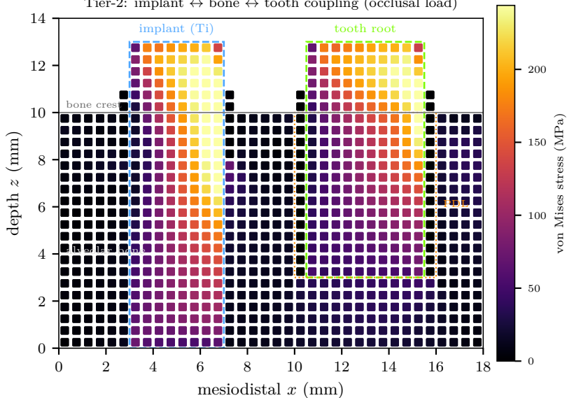
Tier-2: implant \leftrightarrow bone \leftrightarrow tooth coupling (occlusal load)
