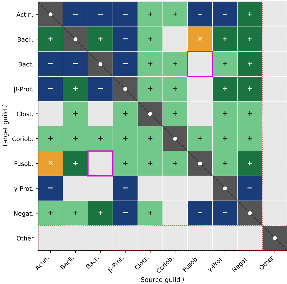
C L1+L2 + AGORA directed / asymmetric (gLV style — no symmetry constraint) 57/90 directed pairs constrained (+:40 -:17 free:31/90)
