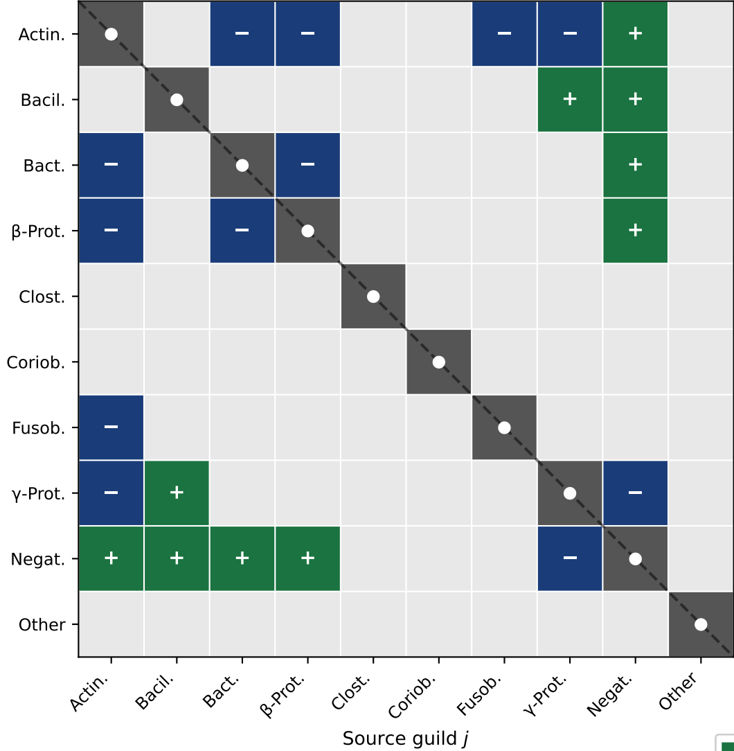
A L1+L2 prior only (+: 5 pairs, -: 6 pairs | constrained: 11/45 undirected)
