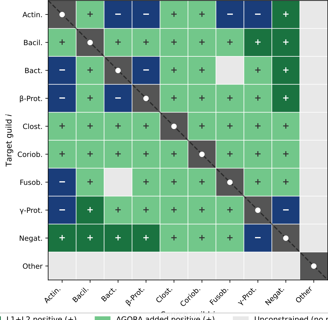
B L1+L2 + AGORA (W=1.0) (AGORA added: +24, -0 | constrained: 35/45 undirected)
