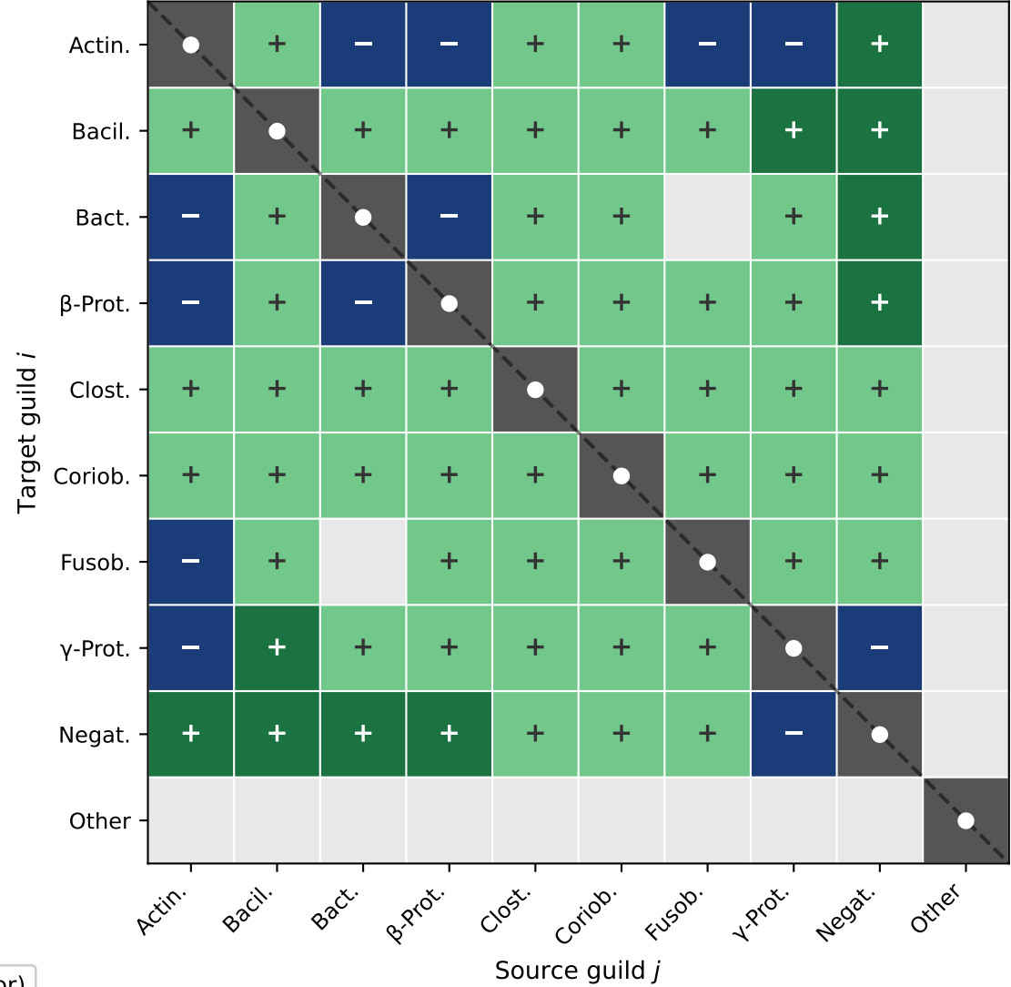
C Remaining unconstrained (grey: 10/45 undirected pairs | no sign prior)
