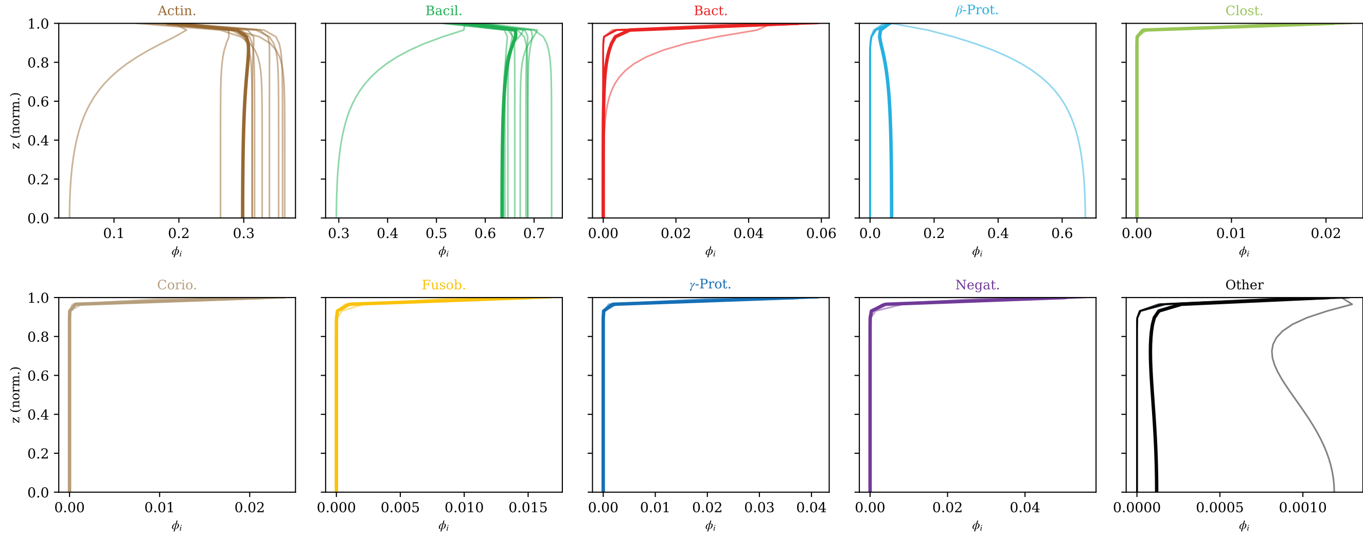
gLV PDE depth profiles at t=21 d — 10 LOO folds (thin) + mean (bold)
