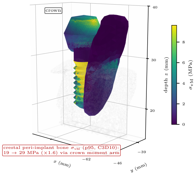
(B) occlusal von Mises \sigma_{vM} ( \sigma_{vM} crown included)
