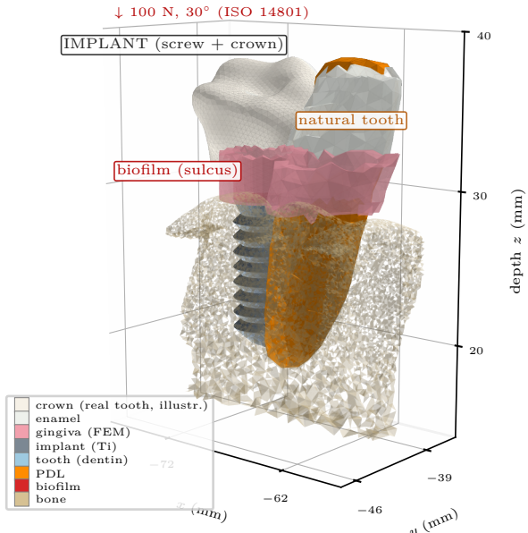
(A) restored implant: load-bearing ceramic crown
