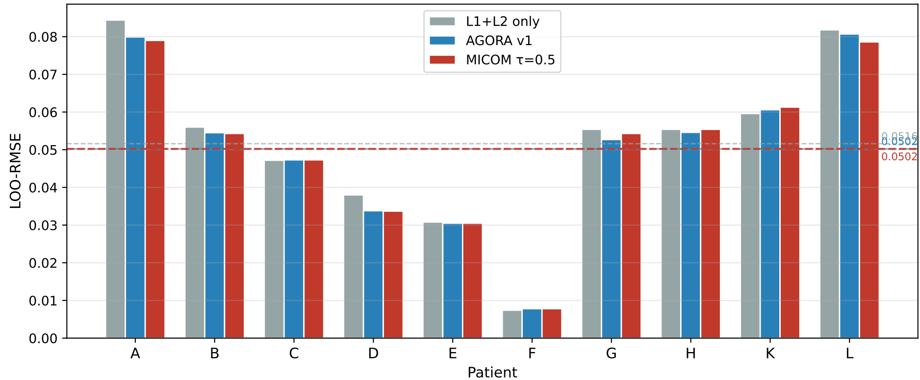
Hamilton Model: Per-Patient LOO-RMSE (L1+L2 vs AGORA v1 vs MICOM)
