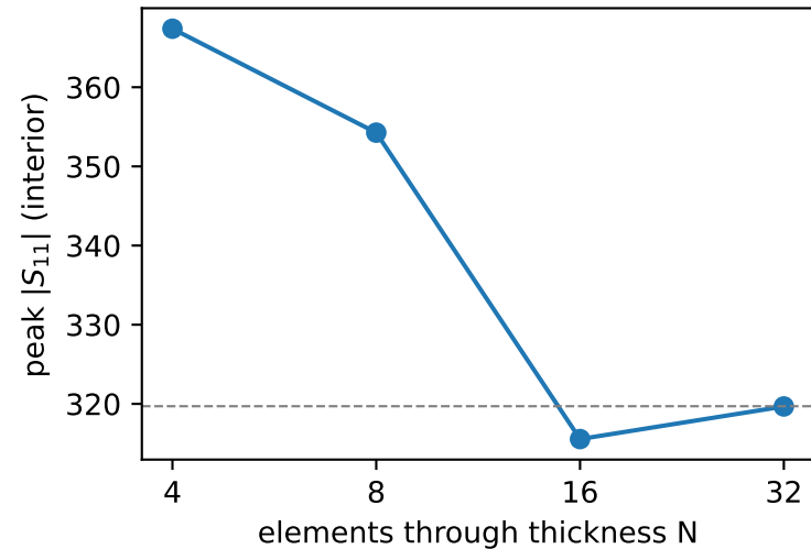
Interior residual stress: CONVERGED (N=16 vs 32: 1.3%)
