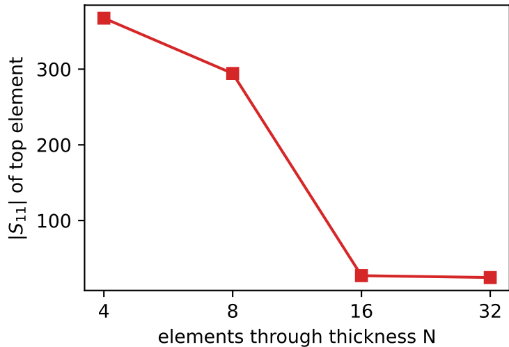
Top element: free-surface boundary layer (not a metric)
