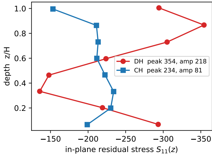
Result: residual stress (FEM)
