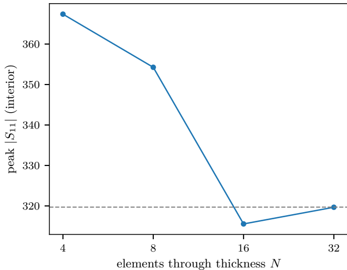
Mesh convergence (N=16 vs 32: 1.3%)
