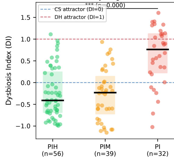
Guild Dysbiosis Index: Szafranski 127 samples (Kruskal-Wallis p=0.000 ) (A) DI by diagnosis (B) LEWIS attractor profiles (Heine et al., last 2 timepoints)
