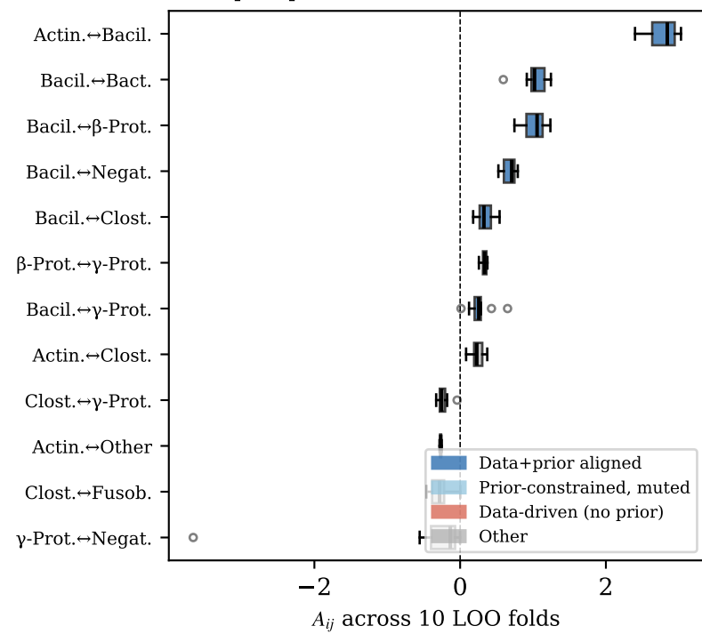
(C) Top 12 pairs: fold-to-fold distribution
