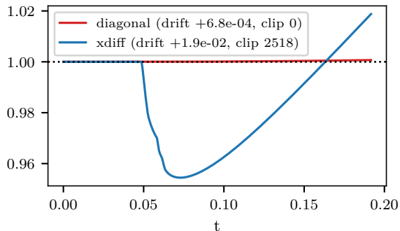
Total mass / M_0 — crowded IC
