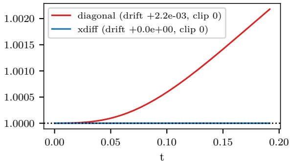
Total mass / M_0 — crowded IC
