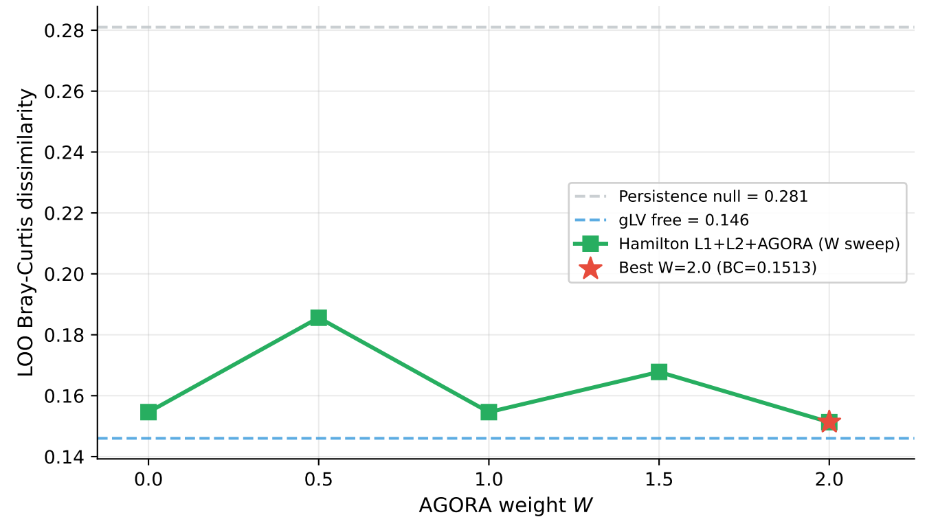
B AGORA weight sensitivity — Bray-Curtis (lower is better)
