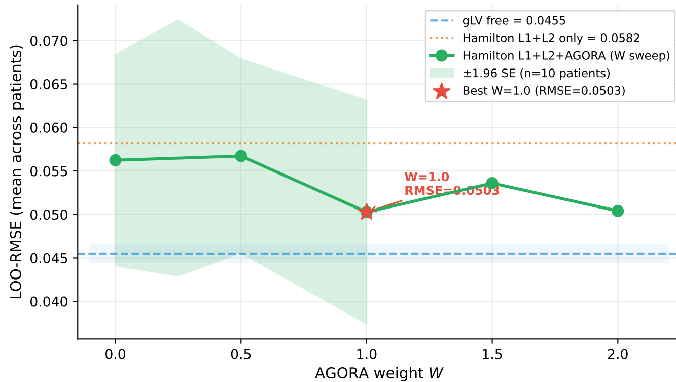
A AGORA weight sensitivity — LOO-RMSE (lower is better; dashed = baselines)
