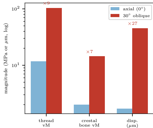
(C) oblique load dominates (ISO 14801)
