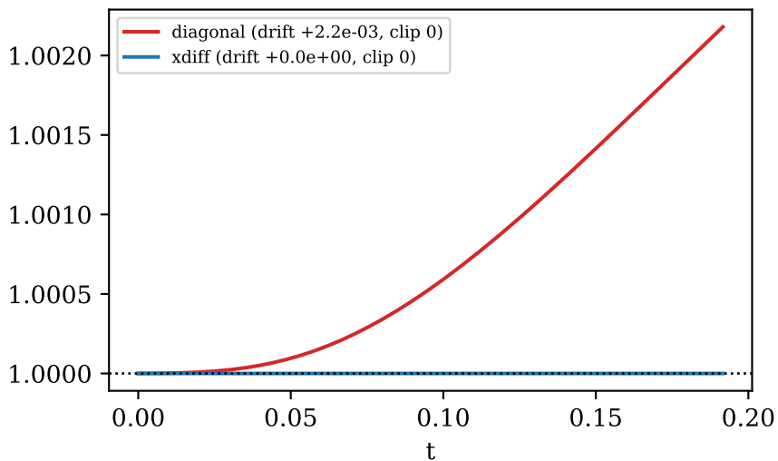
Total mass / M_0 — sub-critical IC
