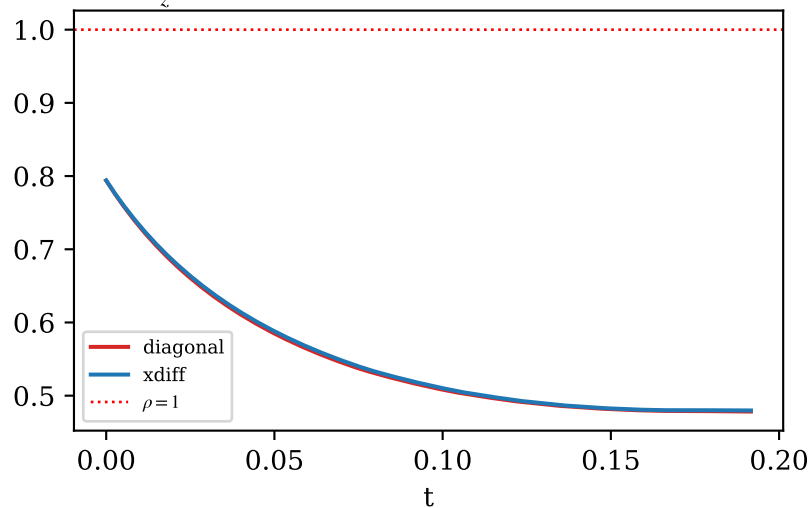
\max \rho — sub-critical IC (IC max 0.80)
