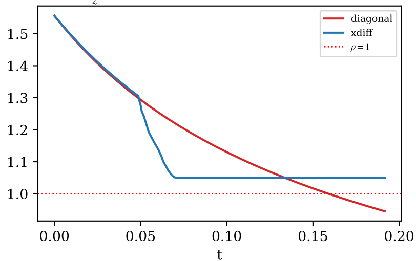
\max \rho — crowded IC (IC max 1.56)
