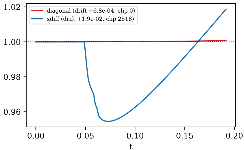
Total mass / M_0 — crowded IC
