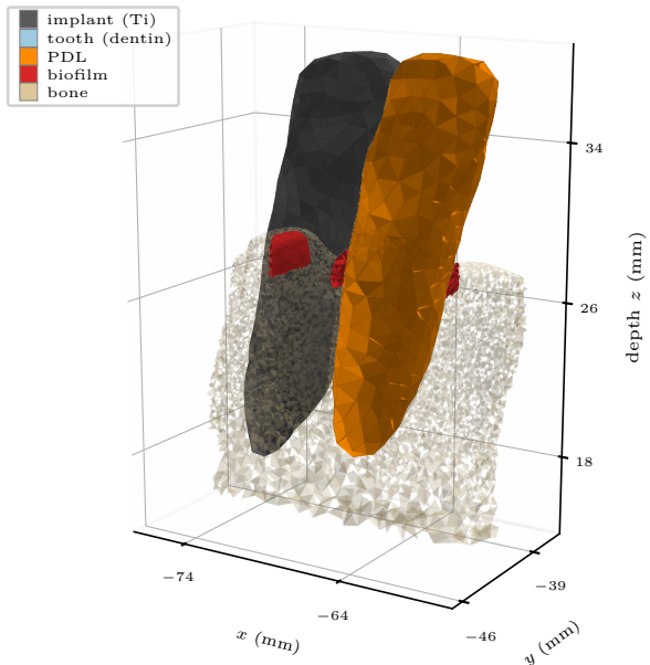
(A) anatomy: real mesh, front bone clipped
