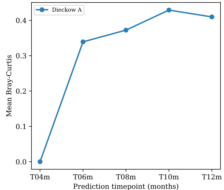
(C) Prediction accuracy over time (BC from observed)
