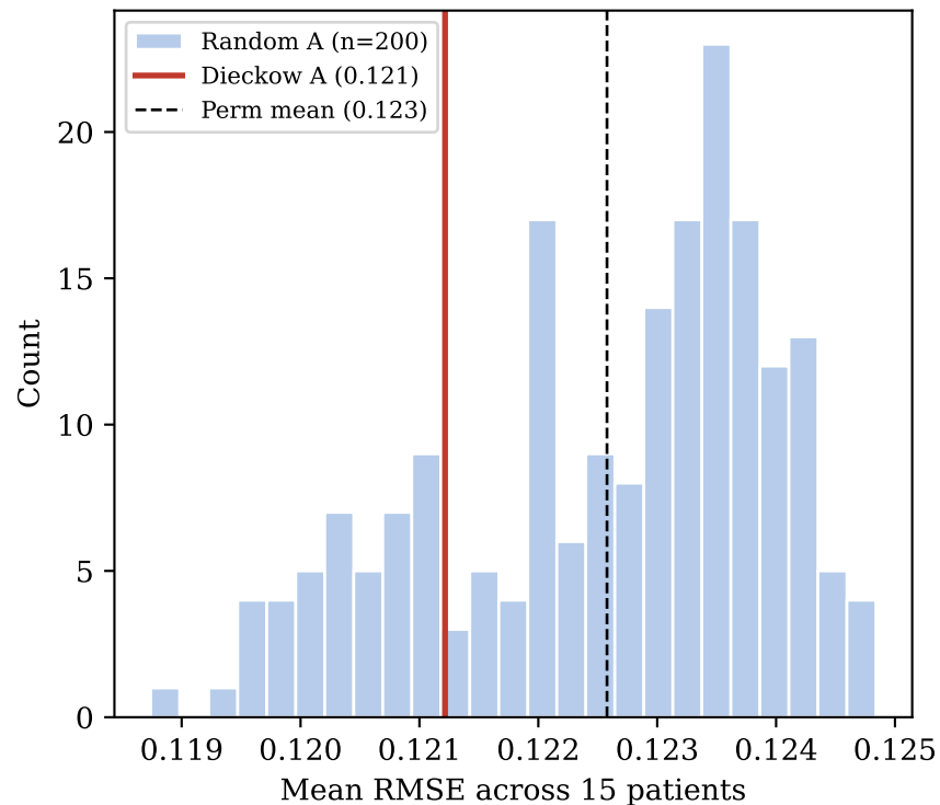
(B) A matrix permutation test (RMSE; p=0.220 )
