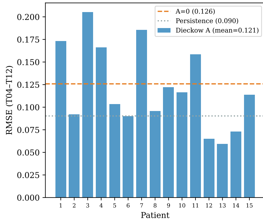
(A) Per-patient prediction RMSE (train on T00-T02, predict T04-T12)
