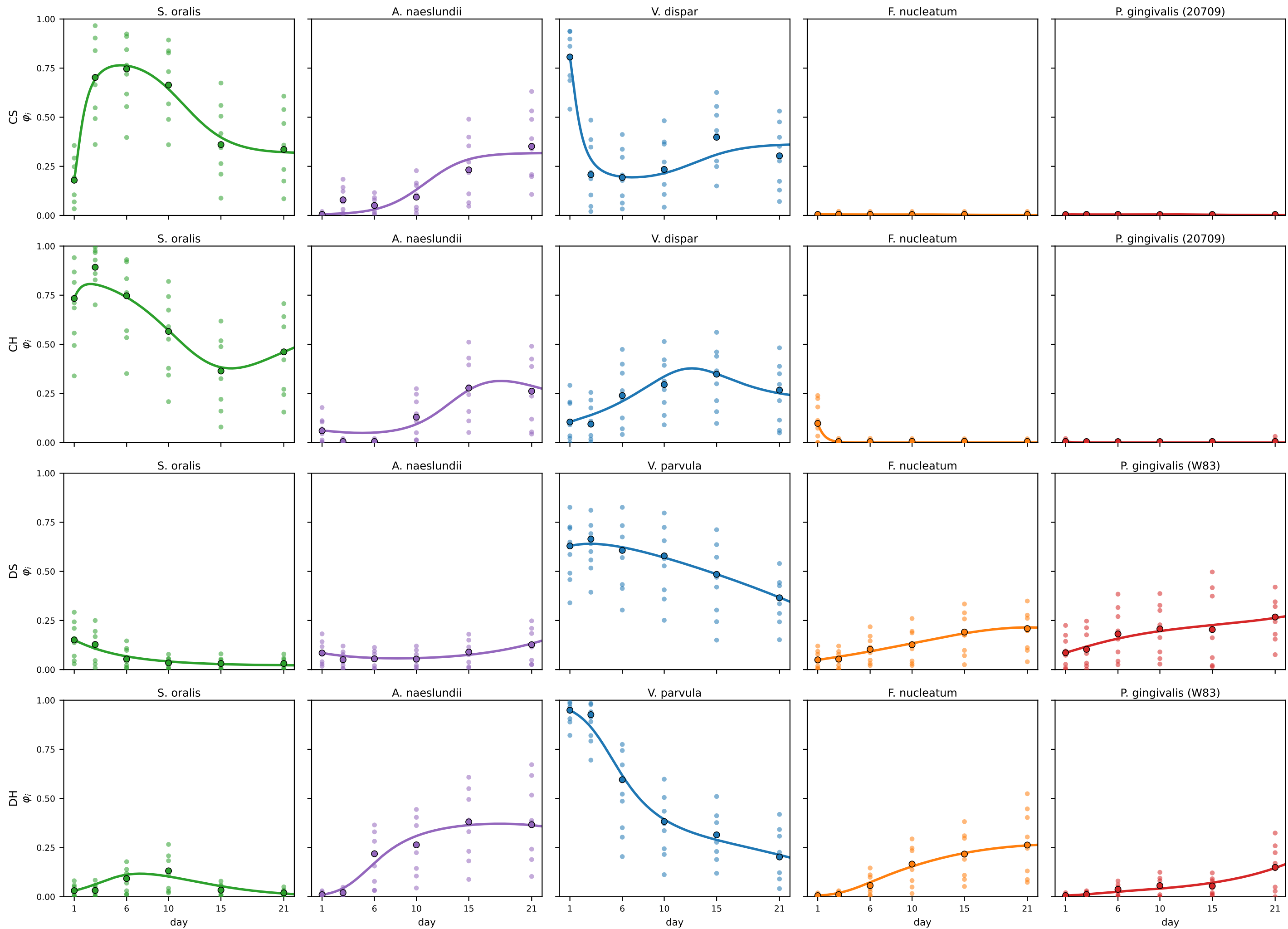
gLV ODE continuous trajectories vs Heine 2025 replicates (CS / CH / DS / DH)
