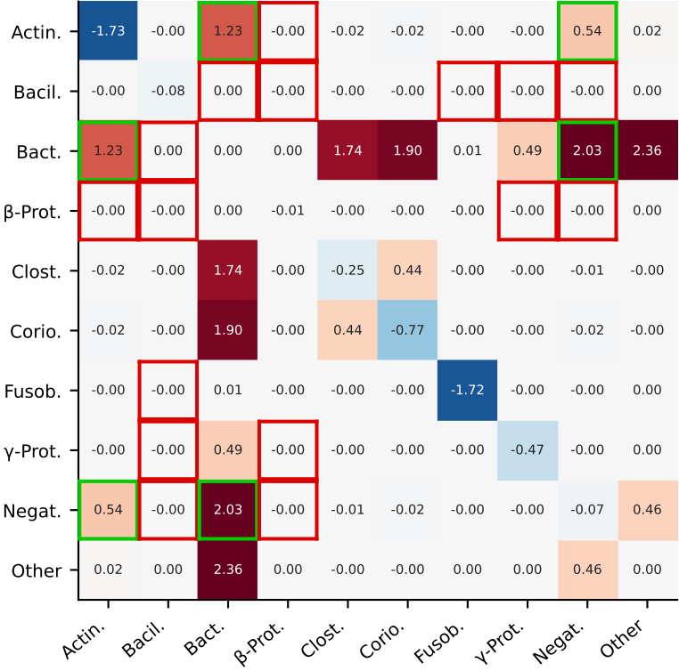
Hamilton — free prior (warm start for KEGG fit)
