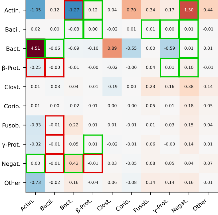
gLV + KEGG prior (reference)
