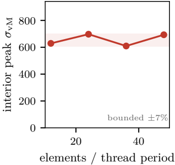
(B) Mesh convergence
