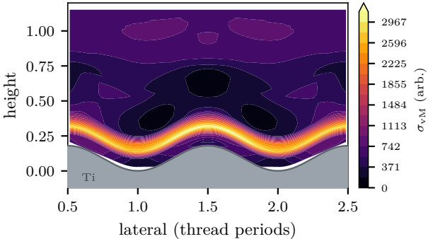
(A) DH interface stress field (stress concentrates at the bonded thread)
