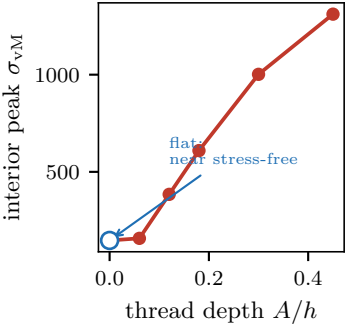
(C) Thread generates the stress
