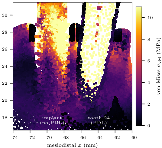
(B) occlusal load: shared-bone coupling
