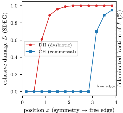
Interface damage at full growth ( t_n^0 = 120 )
