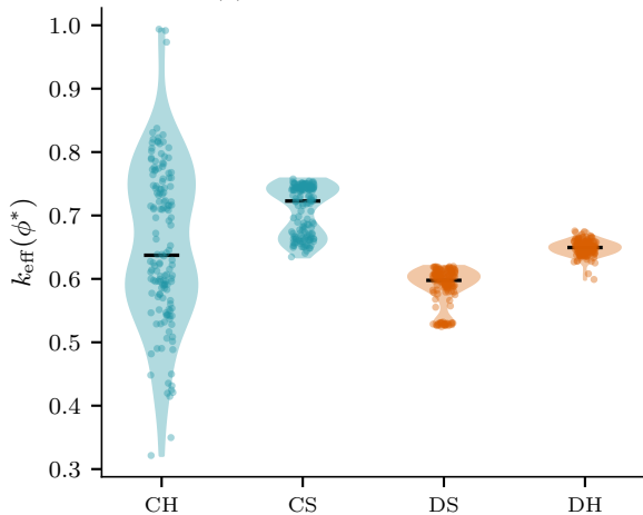
(b) Effective growth rate at \phi^*
