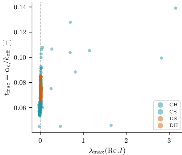
(a) Ecological stability vs fracture time
