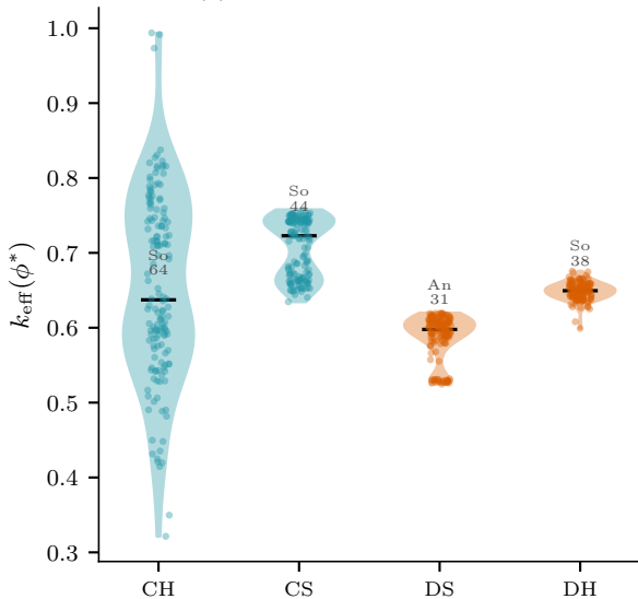
(b) k_{\text{eff}} distribution per condition
