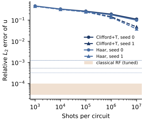
(a) Error vs shots (dotted: exact)
