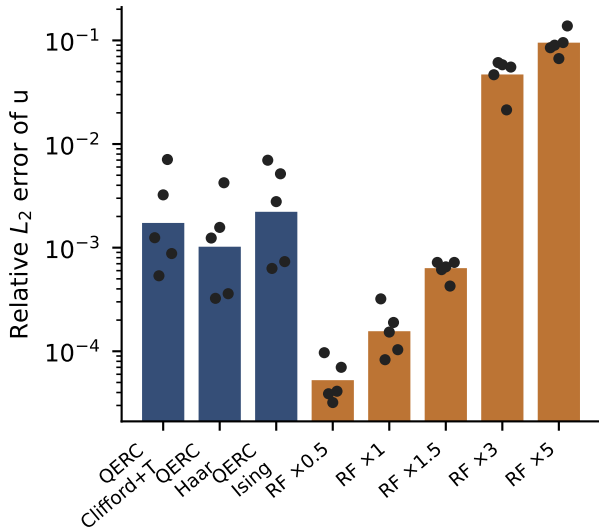
(a) Kirsch, PDE only, N=10 , 5 seeds
