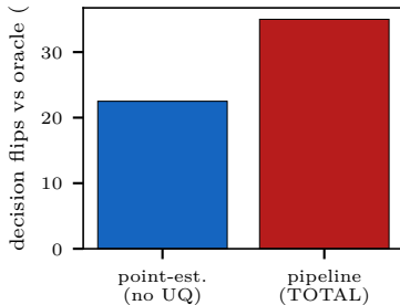
(b) error decomposition dangerous-miss 0
