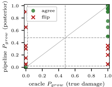
(a) SRB-3 decisions vs truth acc=65
