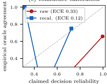
(c) confidence calibration
