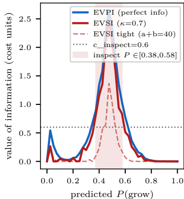
(a) VoI peaks in the ambiguous mid-band
