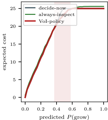
(b) VoI tracks the lower cost envelope
