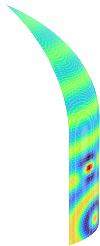
H3 fairing
