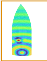
guided-wave field
