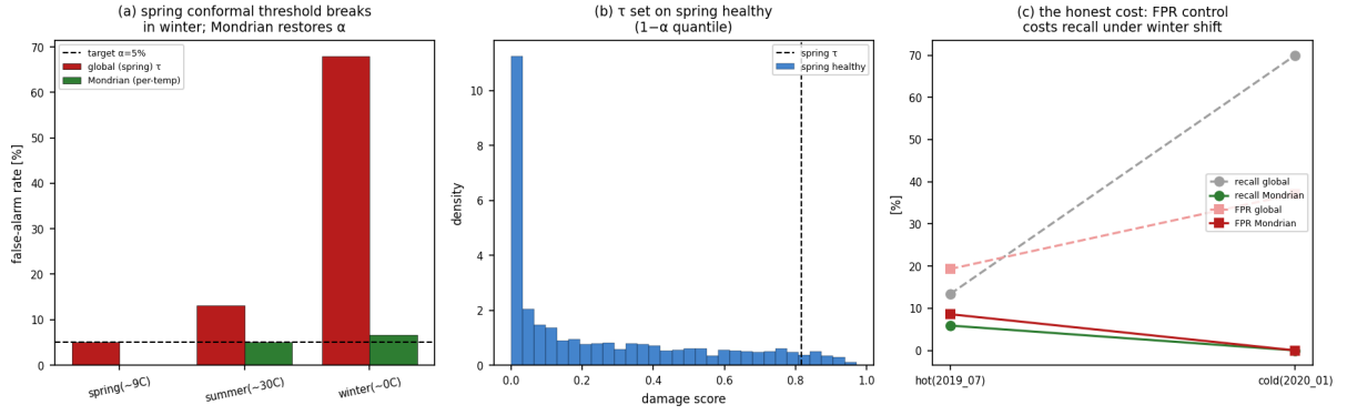
Figure 15: Conformal clearance guarantee under the real seasonal shift (fairing, OGW long-term). (a) a spring-calibrated split-conformal false-alarm threshold holds in distribution but the winter shift inflates the false-alarm rate to \sim 68\% at a nominal 5\% ; a temperature-conditional (Mondrian) threshold restores \approx \alpha across seasons. (b) the spring healthy-score calibration. (c) the honest cost: under the strong winter shift, restoring false-alarm control by recalibration alone collapses cold-damage recall — the shift degrades separability, so feature-level domain adaptation, not recalibration, recovers detection power.
