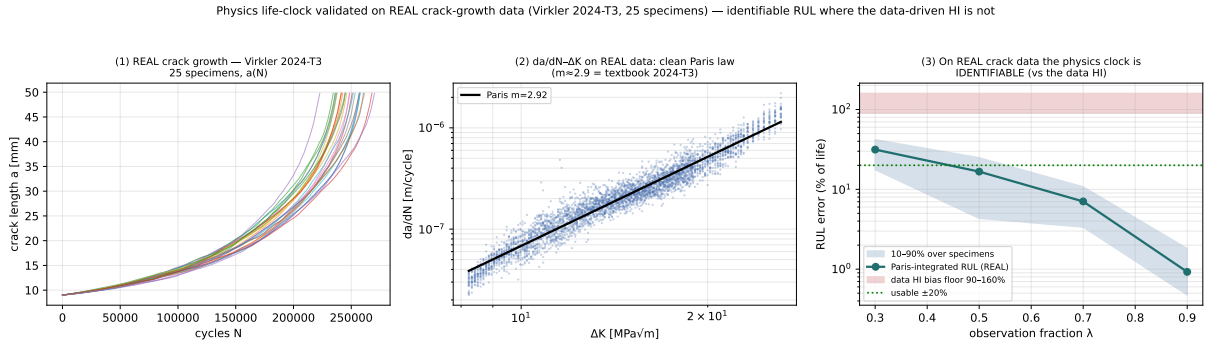
Figure 8: The physical life-clock is identifiable on real crack growth (Virkler 2024-T3, 25 specimens): (left) measured a(N) ; (centre) da/dN-\Delta K recovers the textbook Paris law m=2.92 ; (right) leave-the-future-out remaining-life error sharpens with observation (16.7% \rightarrow 0.9% of life), far below the data-driven index’s flat 90–160% floor.
