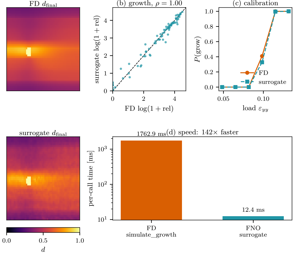
Figure 9: Stage 3 FNO surrogate. FD vs. surrogate damage field, rel_growth agreement, P(\text{grow}) vs. load, and the 142 \times wall-clock speedup.
