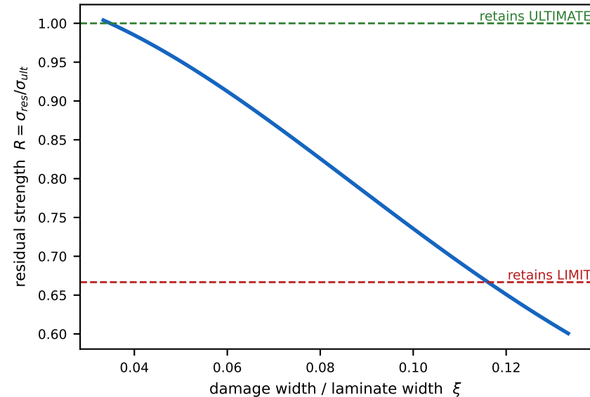
(a) CAI knockdown (BVID design driver) [S1,S4: CMH-17 / ASTM D7136-7]
