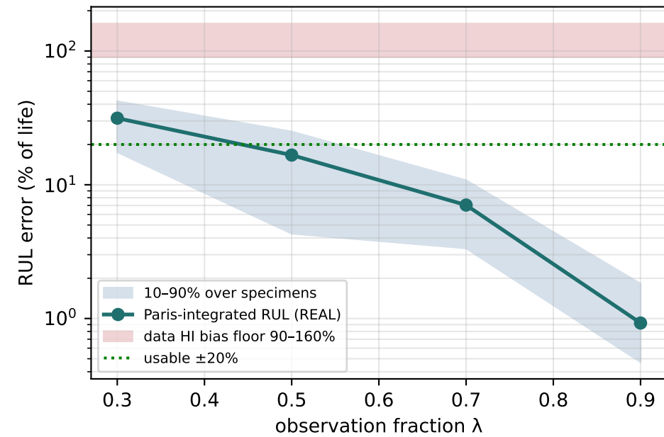
(3) On REAL crack data the physics clock is IDENTIFIABLE (vs the data HI)
