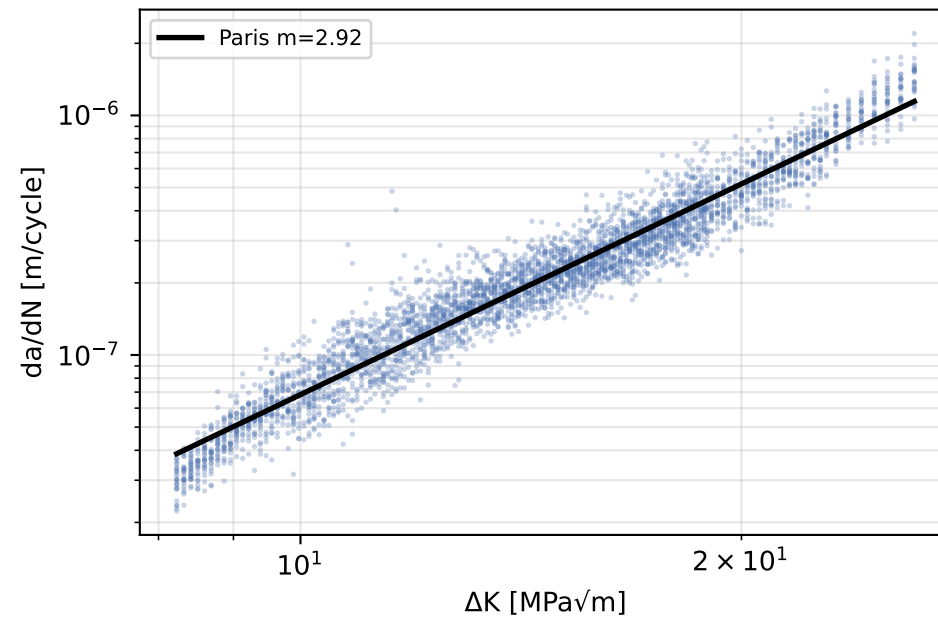
(2) da/dN - \Delta K on REAL data: clean Paris law ( m \approx 2.9 = textbook 2024-T3)
