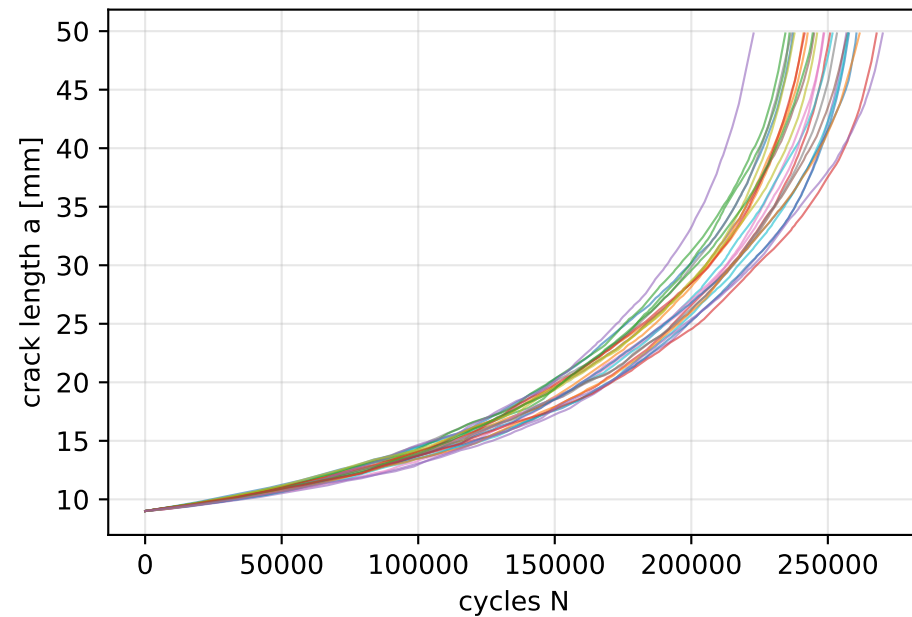
(1) REAL crack growth — Virkler 2024-T3 25 specimens, a(N)
